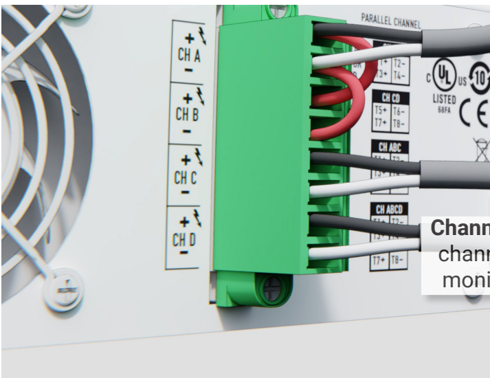
Channel C - Optional channel for single full-range speaker for outside tower.
